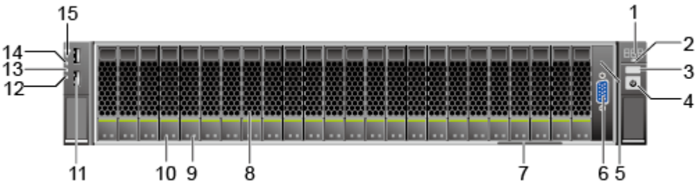
Figure 4-6 Front panel of the RH2288 V3 with 24 hard disks
