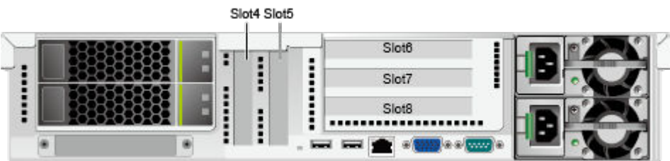
Figure 4-8 PCIe slot layout
