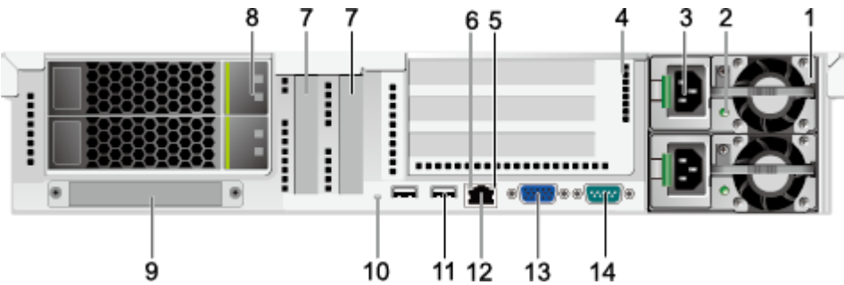
Figure 4-7 Rear panel of the RH2288 V3
