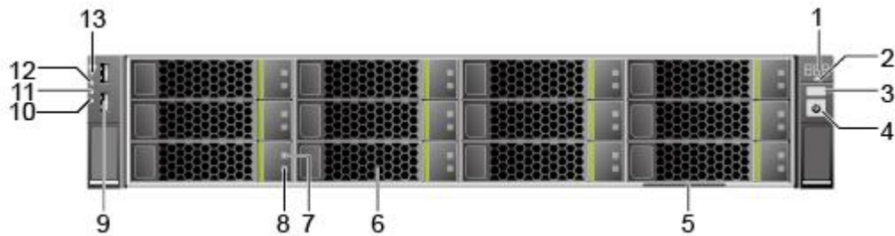
Figure 4-2 Front panel of the RH2288 V3 with 12 hard disks
