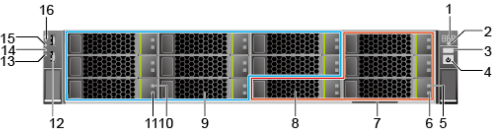
Figure 4-3 Front panel of the RH2288 V3 with twelve 3.5-inch hard disks, including four NVMe PCIe SSDs
