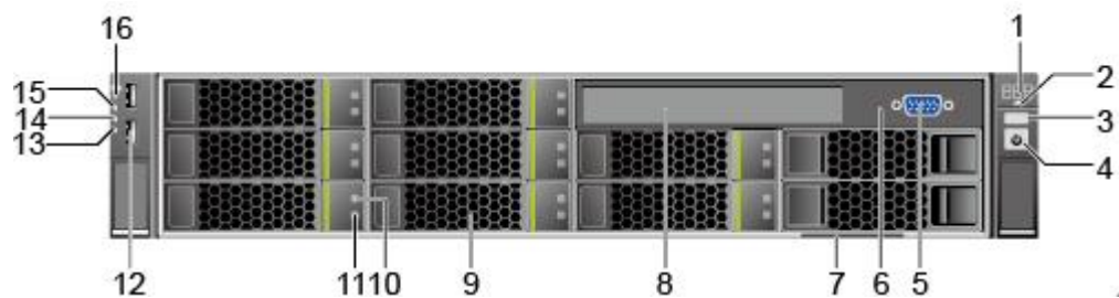
Figure 4-1 Front panel of the RH2288 V3 with eight hard disks
