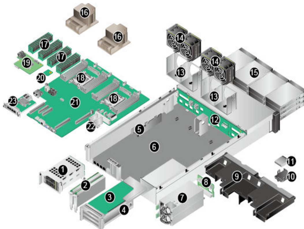
Figure 4-9 RH2288 V3 components
